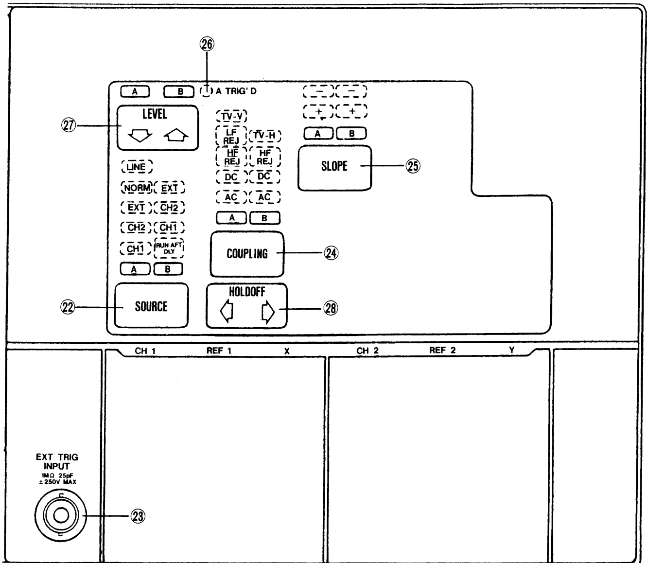
Figure 2-1-3. TRIGGERING
