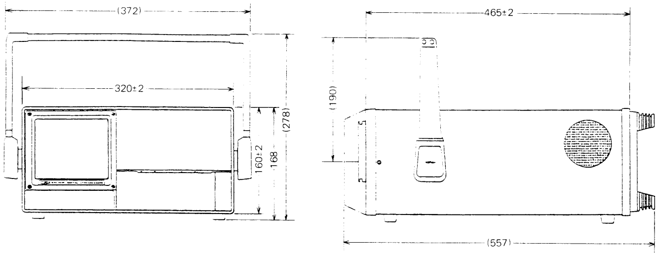
Figure 1-3. Dimensions
